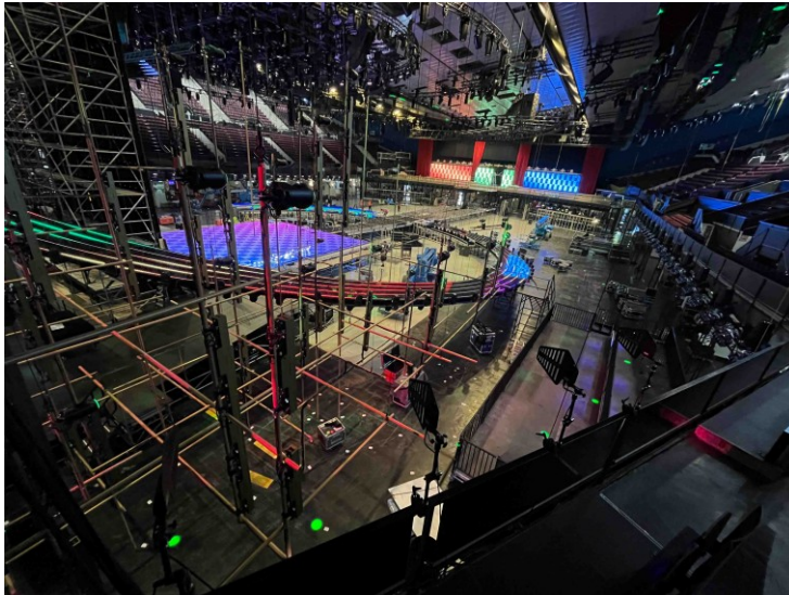
Antenna set-up behind the stage for testing
